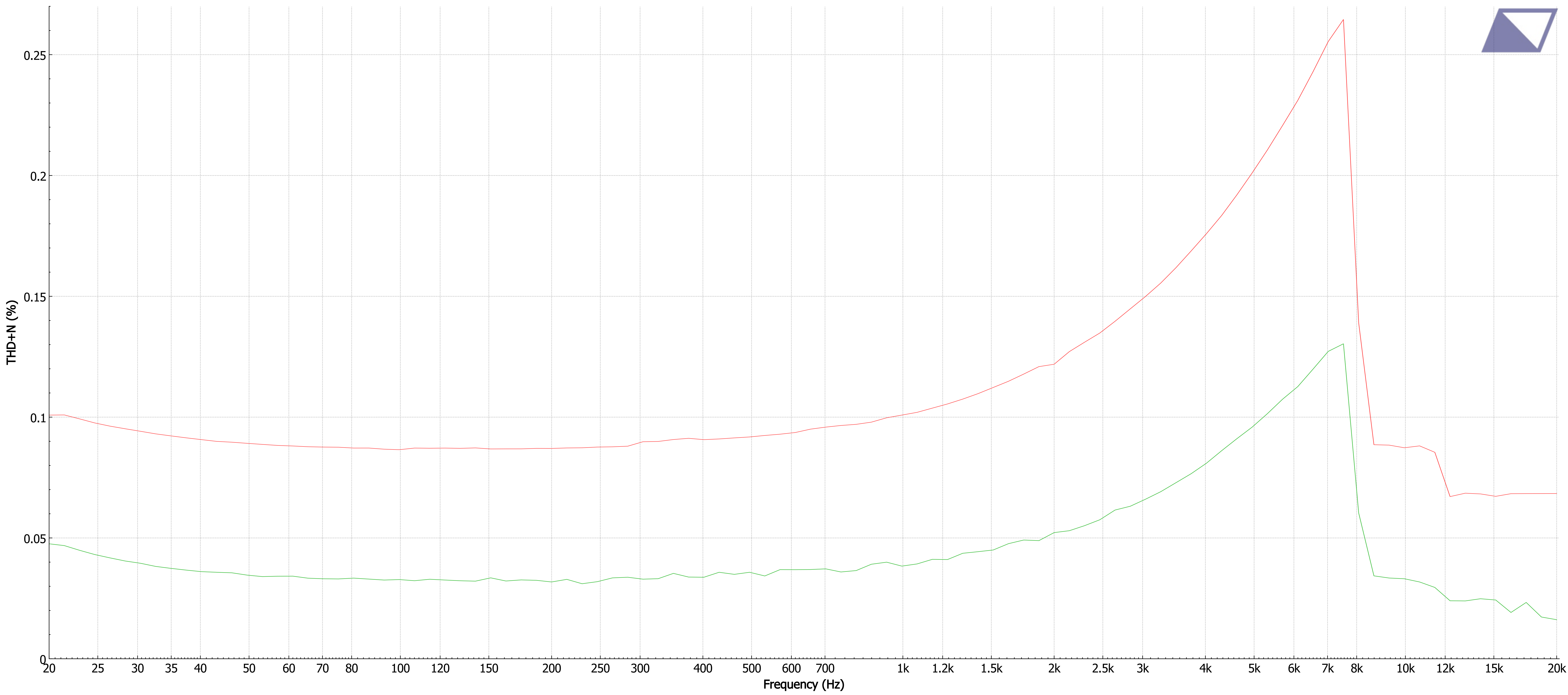
— THD+N (1.5A) - IN (668mV) 20Hz to 20KHZ - OUT (20W) - Analog Unbalanced — THD+N (1.5A) - IN (472mV) 20Hz to 20KHZ - OUT (10W) - Analog Unbalanced
