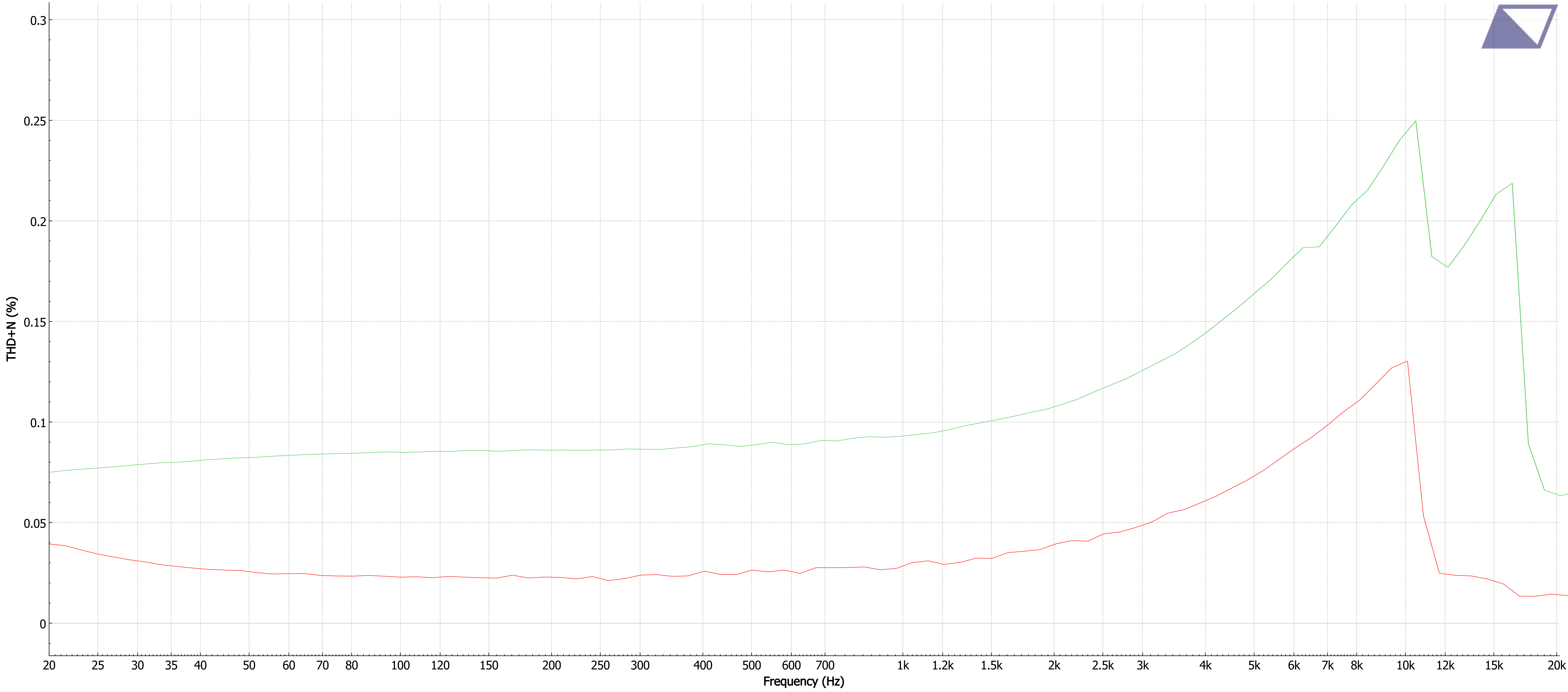
— THD+N (1.5A) - IN (472mV) 20Hz to 20KHZ - OUT (10W) - Analog Unbalanced — THD+N (150mA) - IN (472mV) 20Hz to 20KHZ - OUT (10W) - Analog Unbalanced
