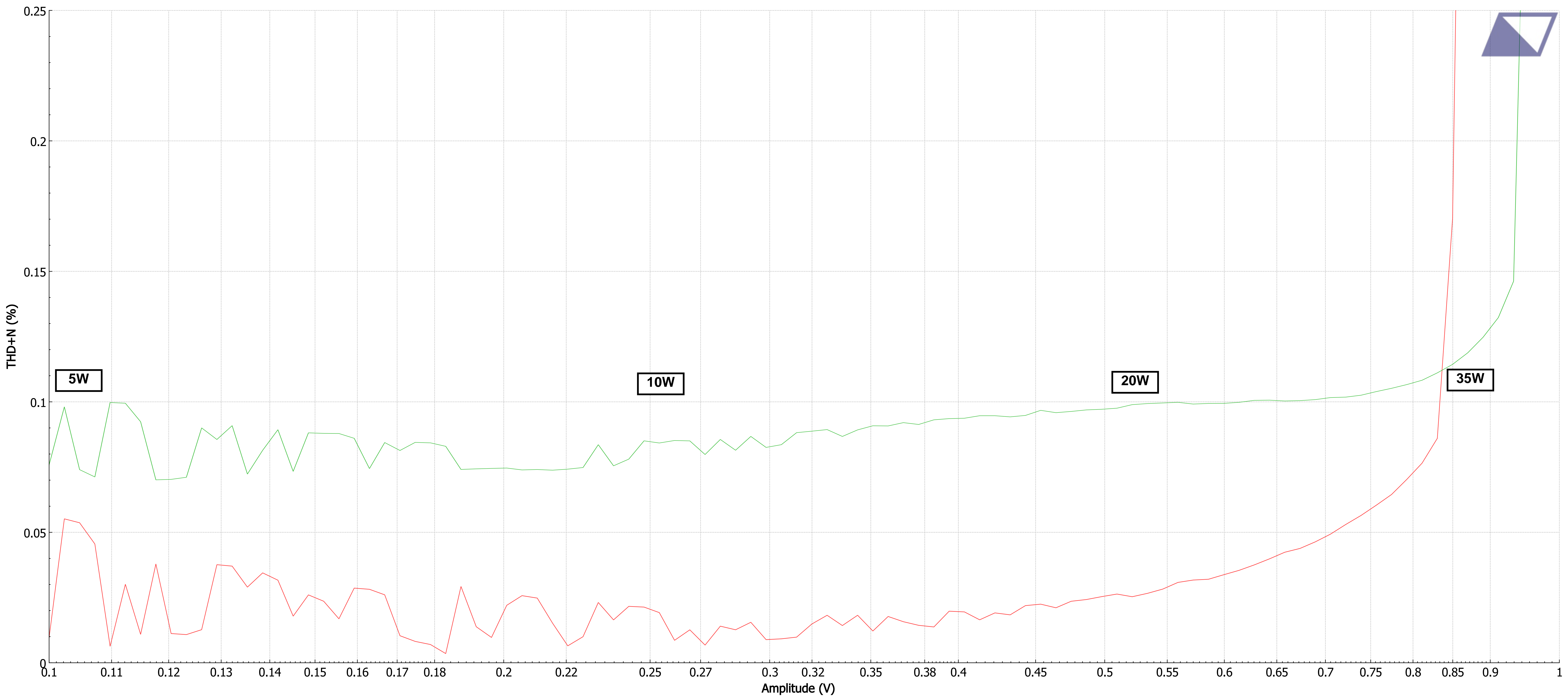
— THD+N (1.5A) - IN (1KHZ) 100mV to 1000mV - Analog Unbalanced — THD+N (150mA) - (1KHZ) 100mV to 1000mV - Analog Unbalanced
