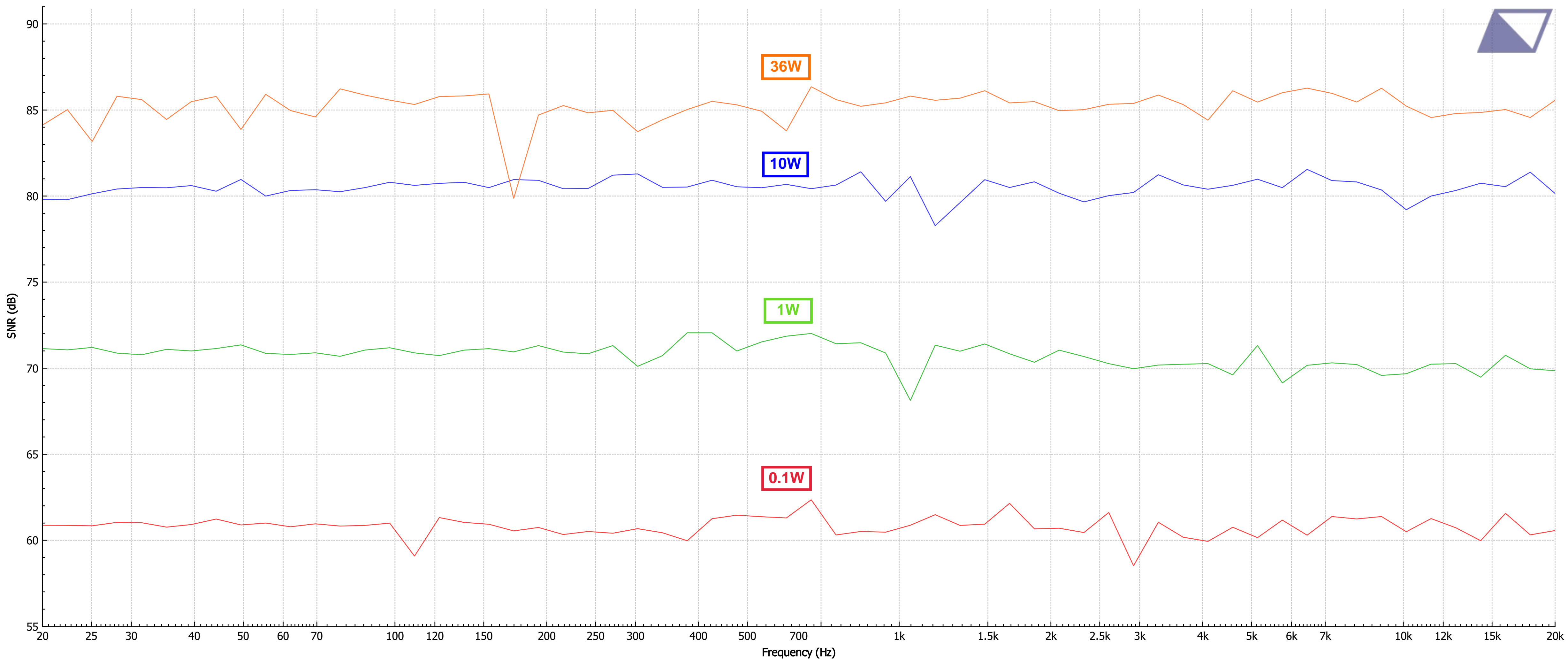
— SNR (150mA) - 20KHz to 22KHz (47mV) - OUT (0.1W) — SNR (150mA) - 20KHz to 22KHz (150mV) - OUT (1W) — SNR (150mA) - 20KHz to 22KHz (472mV) - OUT (10W) — SNR (150mA) - 20KHz to 22KHz (850mV) - OUT (36W)
