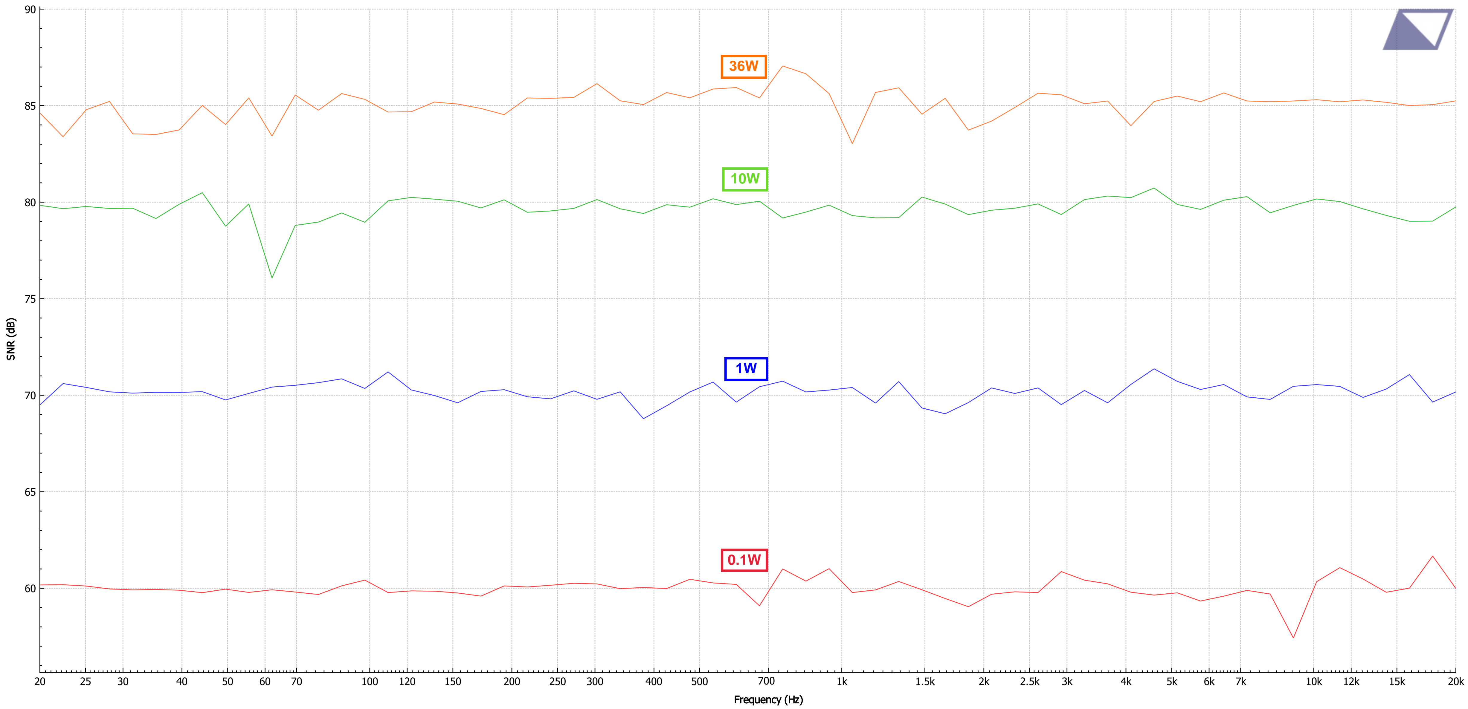
— SNR (1.5A) - 20KHz to 22KHz (47mV) - OUT (0.1W) — SNR (1.5A) - 20KHz to 22KHz (472mV) - OUT (10W) — SNR (1.5A) - 20KHz to 22KHz (150mV) - OUT (1W) — SNR (1.5A) - 20KHz to 22KHz (850mV) - OUT (36W)
