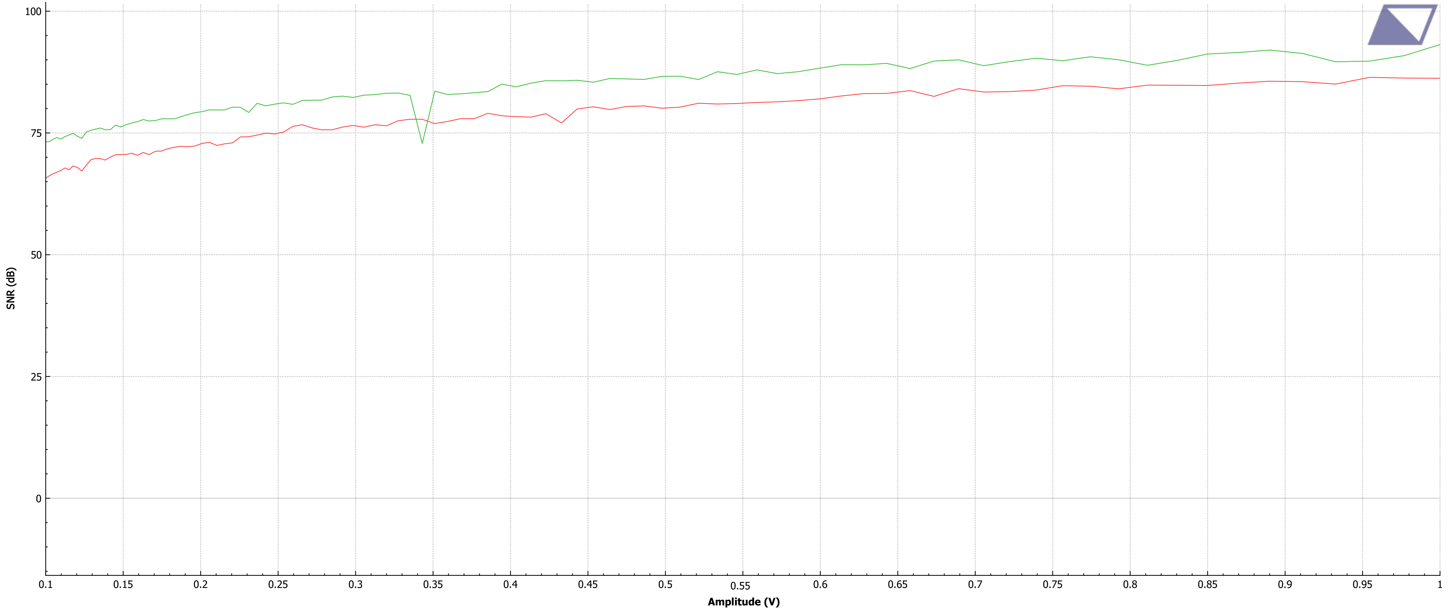
— SNR (1.5A) - 100mV to 1000mV (100HZ) - Analog Unbalanced — SNR (150mA) - 100mV to 1000mV (100HZ) - Analog Unbalanced
