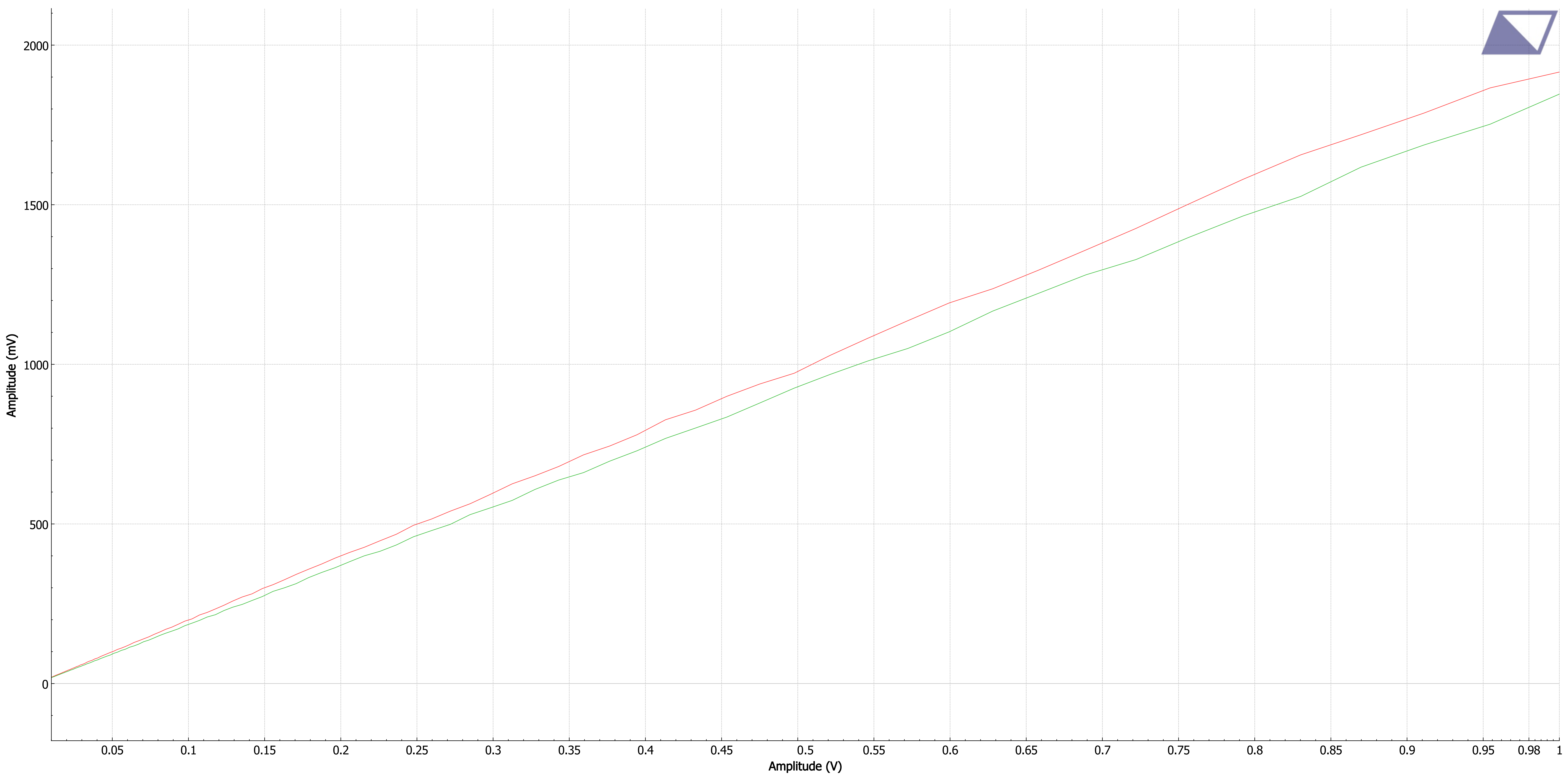
— LEVEL (1.5A) - 1KHZ 10mV to 1000mV - Analog Unbalanced — LEVEL (150mA) - 1KHZ 10mV to 1000mV - Analog Unbalanced
